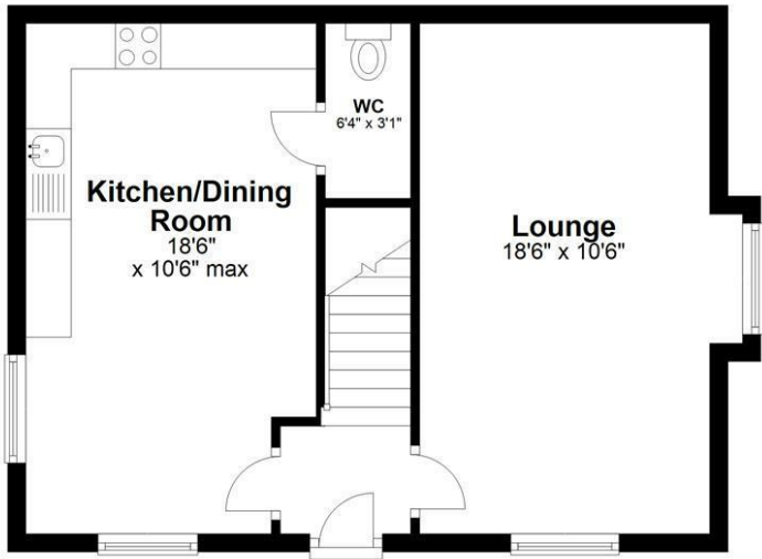
Ground Floor Approx. 463.0 sq. feet
